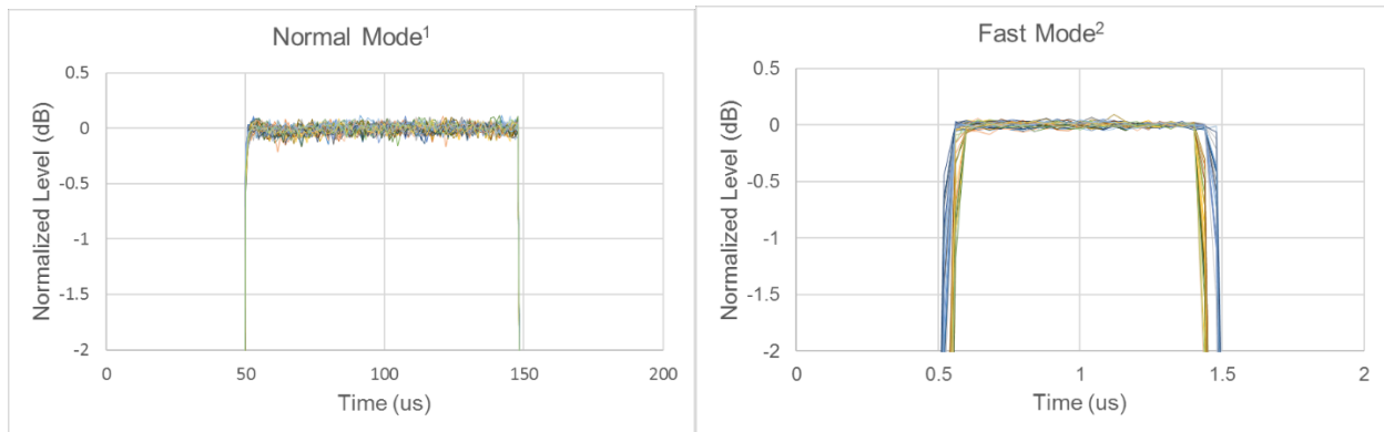
Figure 20. Pulse modulation shape (Normal mode and Fast mode) on E5056A/57A/58A with S96325B, 32 GHz
