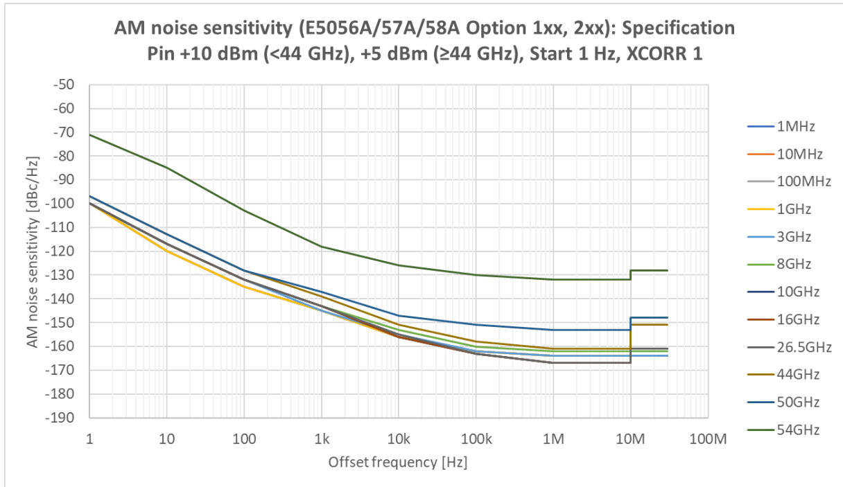
Figure 11. SSB AM noise sensitivity (E5056A/57A/58A Option 1xx, 2xx): Specification, +10 dBm (<44 GHz), +5 dBm (≥ 44 GHz) input, Auto Range OFF, Max. input level = signal level + 3 dB, start offset frequency = 1 Hz, Cross correlation factor = 1
