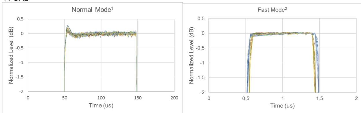
Figure 21. Pulse modulation shape (Normal mode and Fast mode) on E5056A/57A/58A with S96325B, 44 GHz
