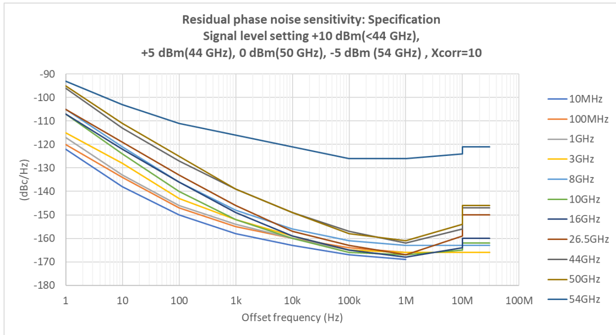
Figure 13. Residual phase noise sensitivity (dBc/Hz) (E5055A/56A/57A/58A): Specification, Cross correlation factor = 10, Fast XCORR mode OFF, signal level setting = +10 dBm(<44 GHz), +5 dBm(44 GHz), 0 dBm(50 GHz), -5 dBm(54 GHz), Auto range OFF, Max. input level = signal level + 3 dB, Path delay compensation 0 sec, start offset = 1 Hz -1
