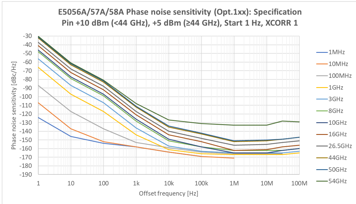
Figure 7. SSB Phase noise sensitivity (E5056A/57A/58A Option 1xx): Specification, +10 dBm (<44 GHz), +5 dBm (≥ 44 GHz) input, Auto Range OFF, Max. input level = signal level + 3 dB, Auto Range On, start offset frequency = 1 Hz, Cross correlation factor = 1)
