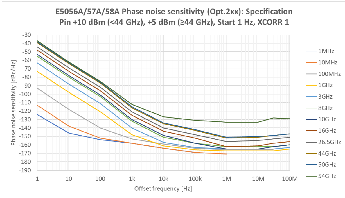
Figure 5. SSB Phase noise sensitivity (E5056A/57A/58A Option 2xx): Specification, +10 dBm (<44 GHz), +5 dBm ( \geq 44 GHz) input, Auto Range OFF, Max. input level = signal level + 3 dB, start offset frequency = 1 Hz, Cross correlation factor = 1)
