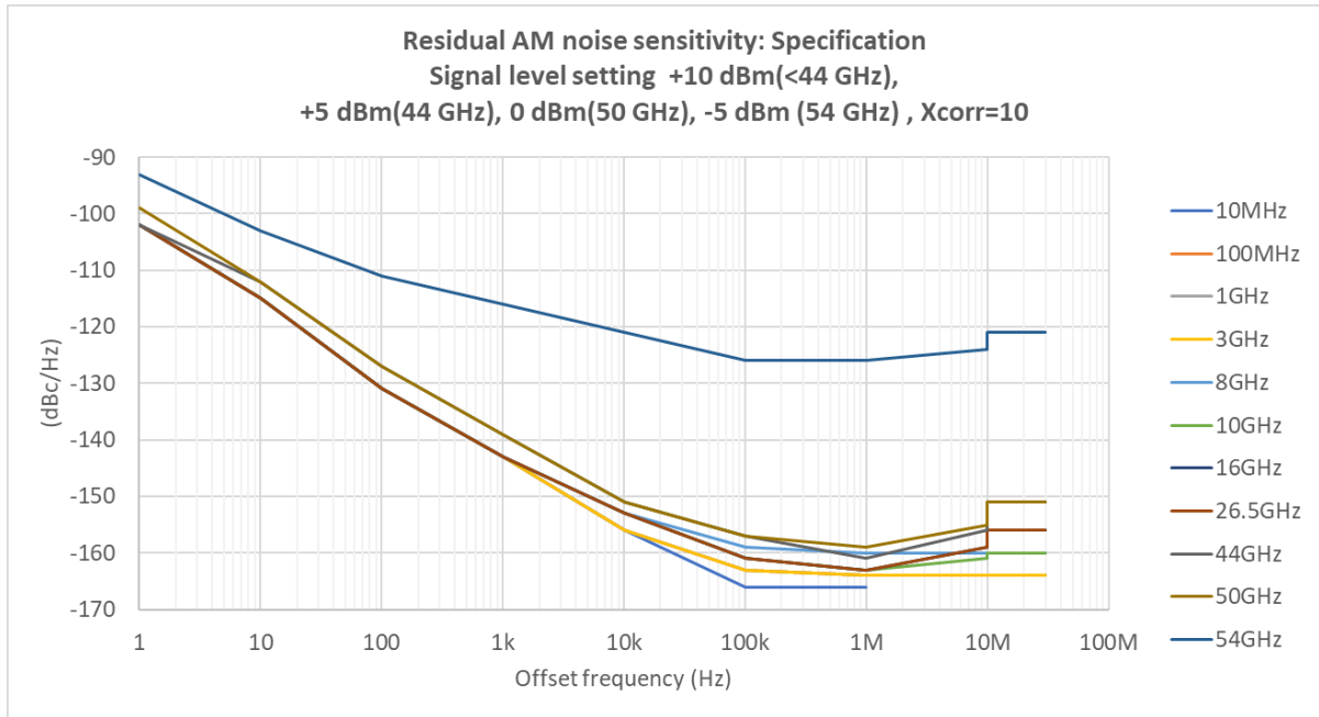
Figure 15. Residual AM phase noise sensitivity (dBc/Hz) (E5055A/56A/57A/58A): Specification, Cross correlation factor = 10, Fast XCORR mode OFF, signal level setting = +10 dBm(<44 GHz), +5 dBm(44 GHz), 0 dBm(50 GHz), -5 dBm(54 GHz), Auto range OFF, Max. input level = signal level + 3 dB, Path delay compensation 0 sec, start offset = 1 Hz 1
