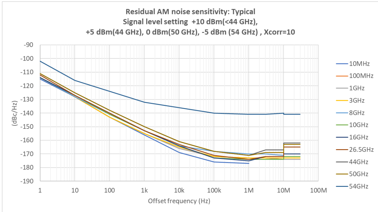
Figure 16. Residual AM phase noise sensitivity (dBc/Hz) (E5055A/56A/57A/58A): Typical, Cross correlation factor = 10, Fast XCORR mode OFF, signal level setting = +10 dBm(<44 GHz), +5 dBm(44 GHz), 0 dBm(50 GHz), -5 dBm(54 GHz), Auto range ON, Path delay compensation 0 sec, start offset = 1 Hz 1
