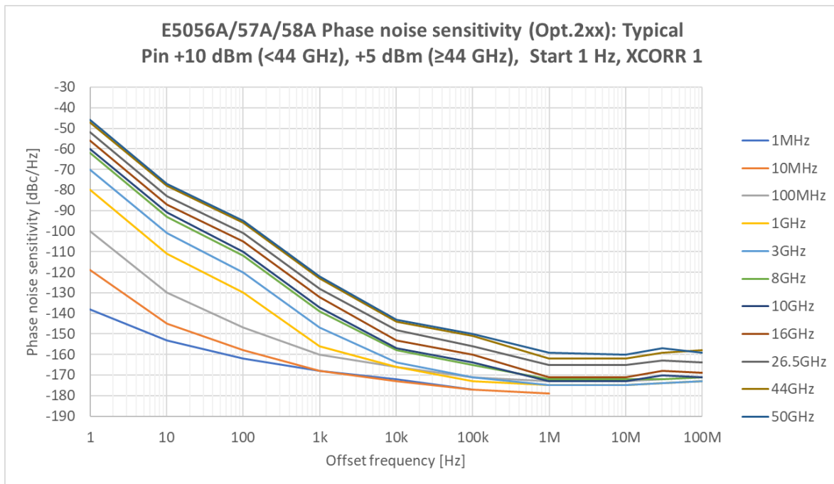
Figure 6. SSB Phase noise sensitivity (E5056A/57A/58A Option 2xx): Typical, +10 dBm (<44 GHz), +5 dBm ( \geq 44 GHz) input, Auto Range On, start offset frequency = 1 Hz, Cross correlation factor = 1)
